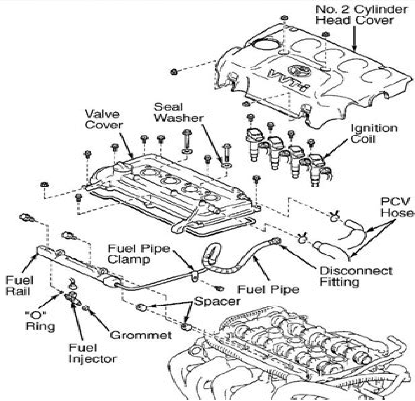
Fig. 66: Exploded View Of Fuel Rail & Components (ECHO)
