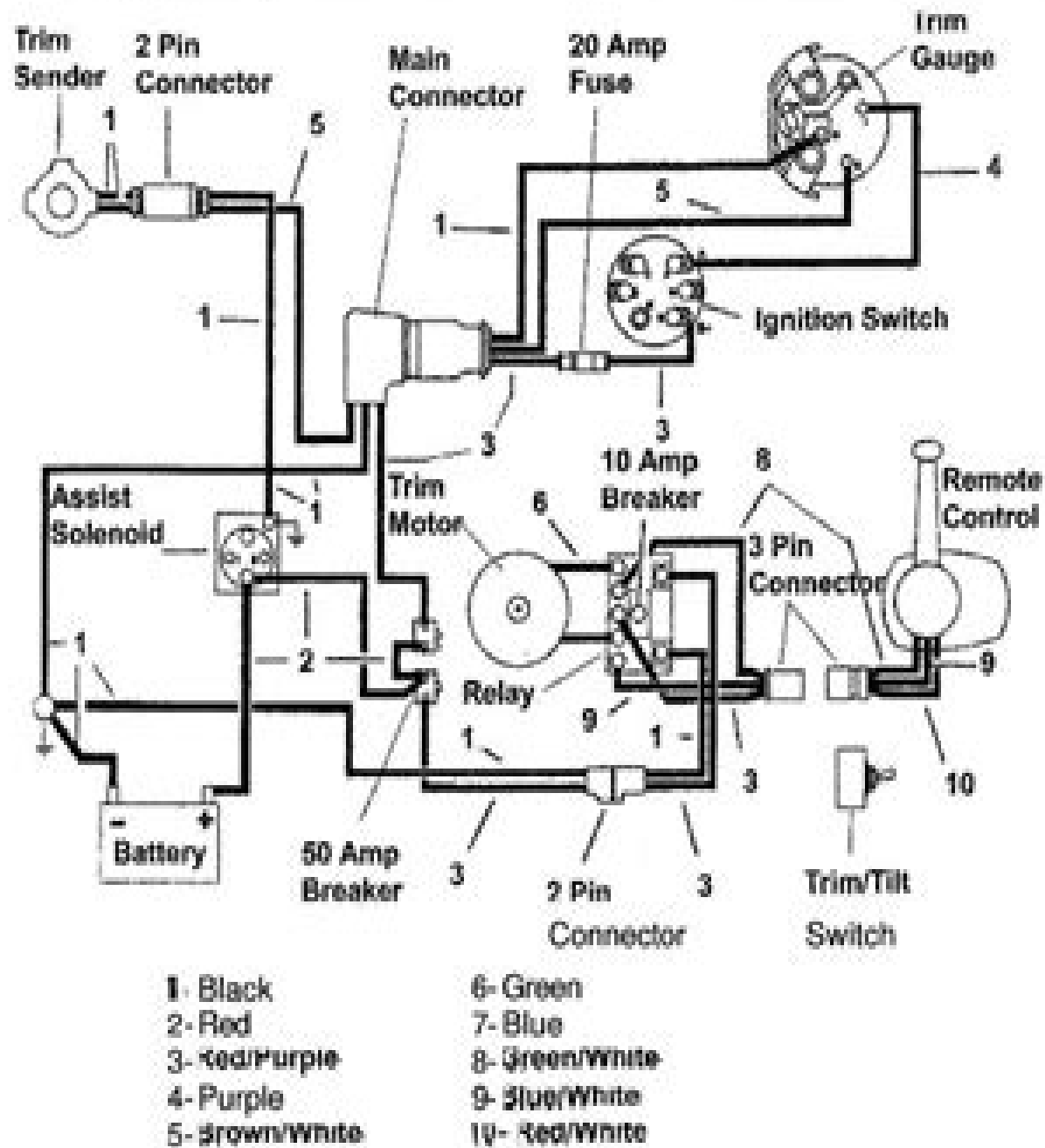
Fig. 101 Power trim/tilt—1991-92 models, 1993 GM models and 1994-95 /4GL GM models
