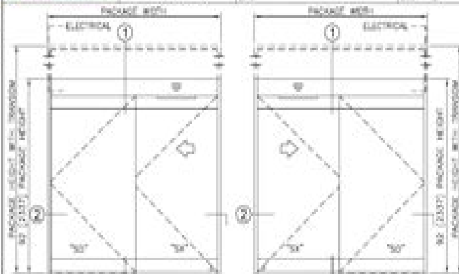
LEFT HAND SIDE ELEVATION VIEW RIGHT HAND SIDE SCALE: 1" = 1'-0"
