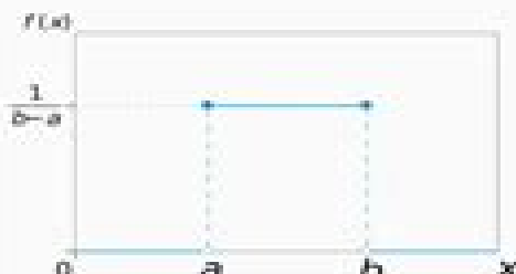
Uniform Distribution
