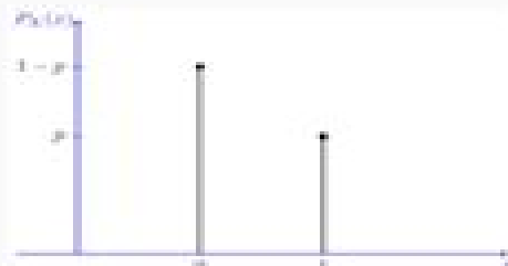
Bernoulli Distribution
