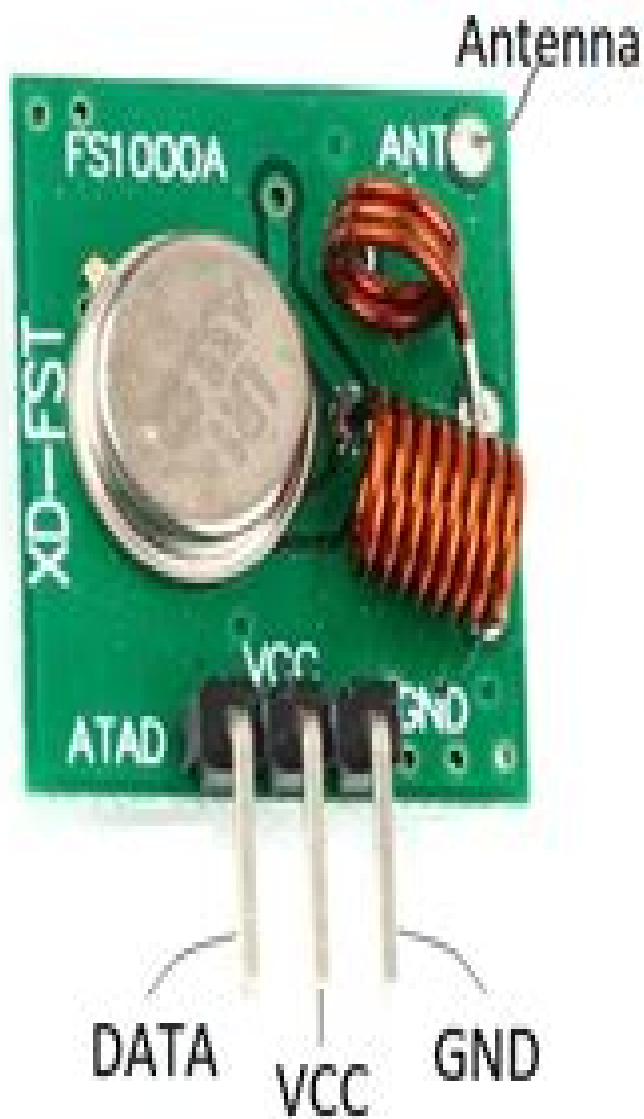
433MHz RF Transmitter
