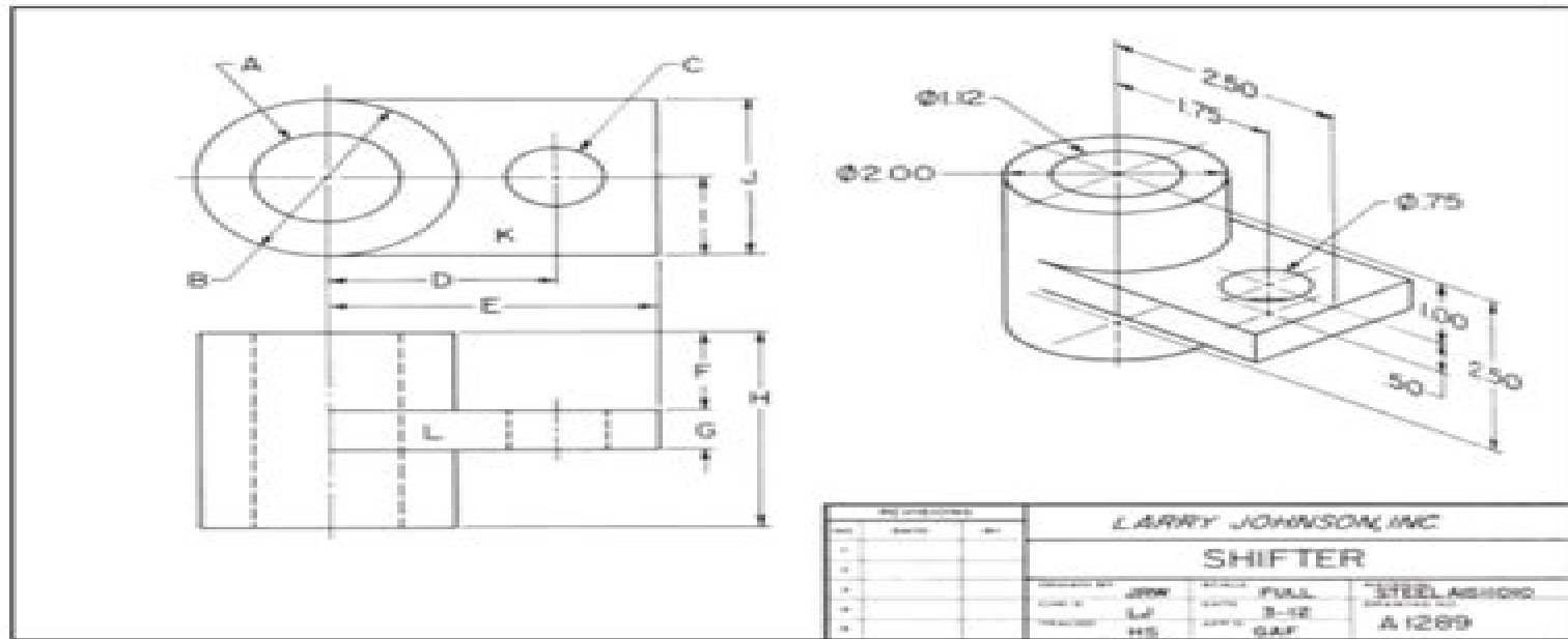
Figure 5-29. Use this print of a shifter to answer questions in Part IV of the Print Reading Activities.
