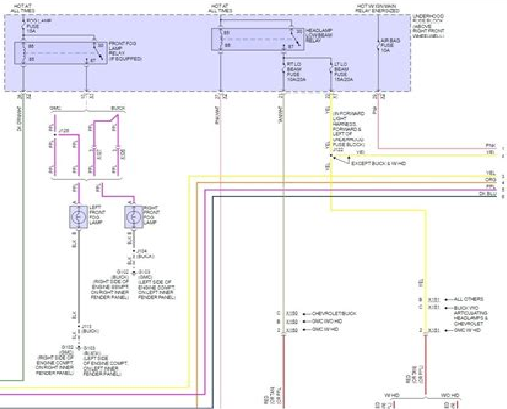
Fig 2: Headlamps Circuit (2 of 3)
