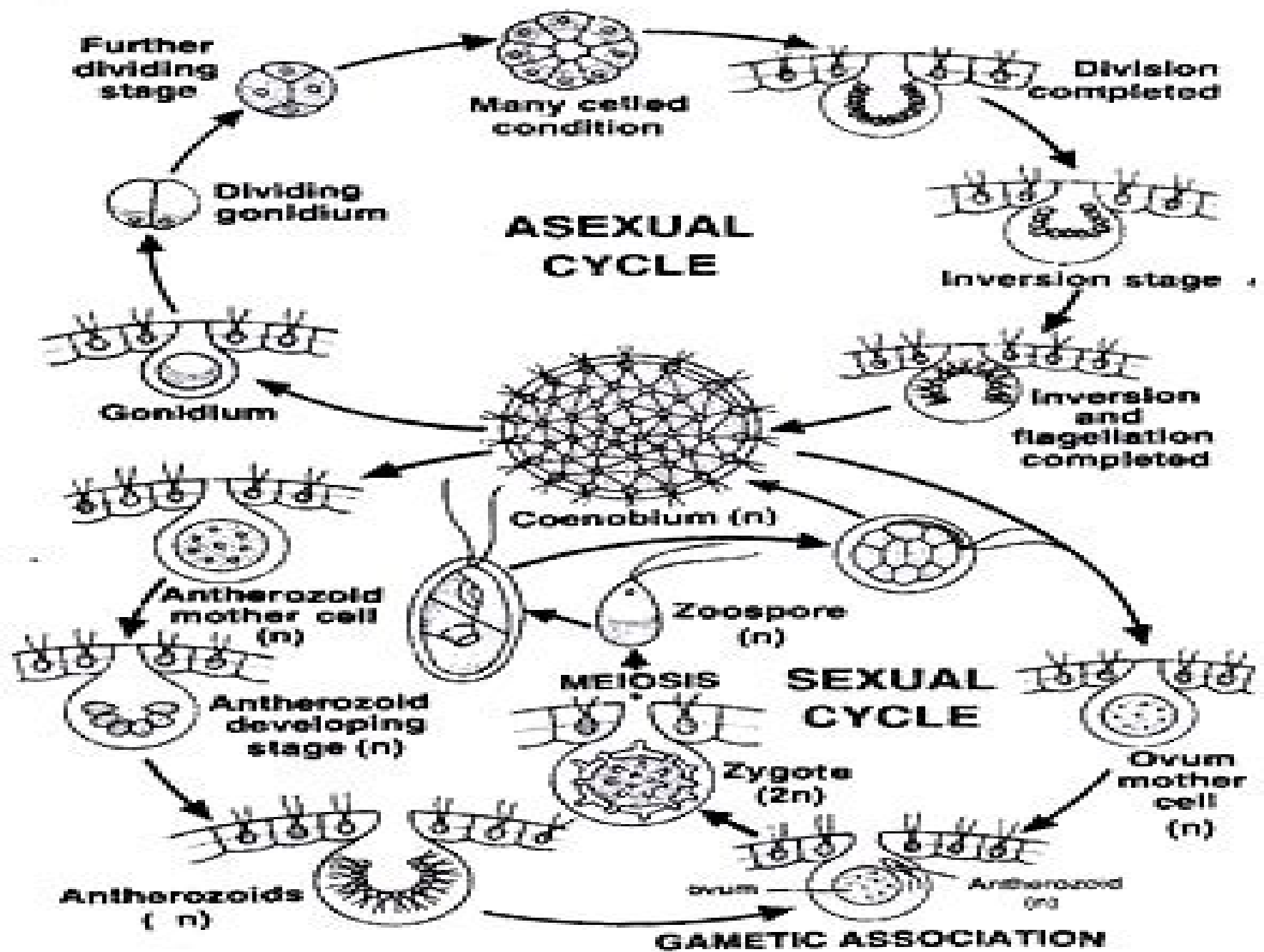
Fig. 7. Volvox . Diagrammatic life cycle.
