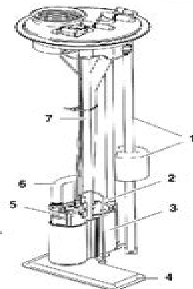
Figure 4-5. Fuel Pump/Filter/Fuel Level Sender Assembly
