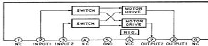
IC802 BUS208
