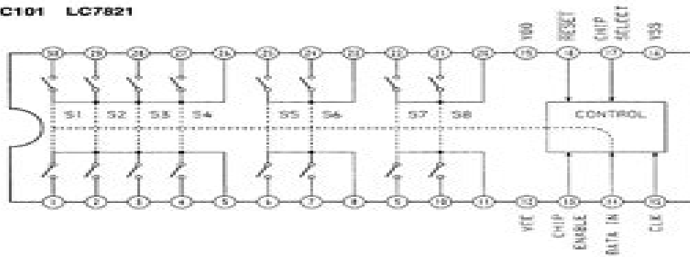
HC101 LC7821
