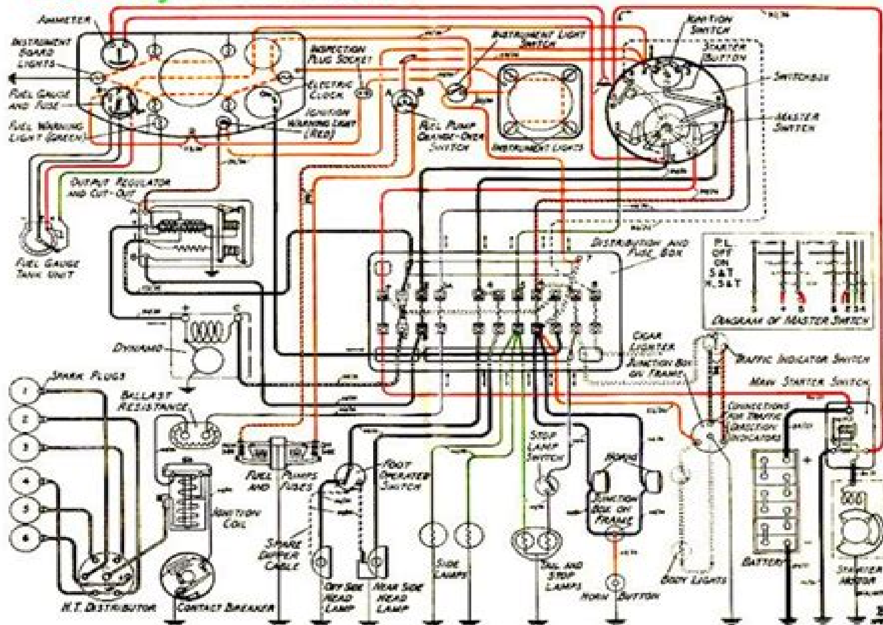
FIG. 35.—ELECTRICAL WIRING DIAGRAM.
