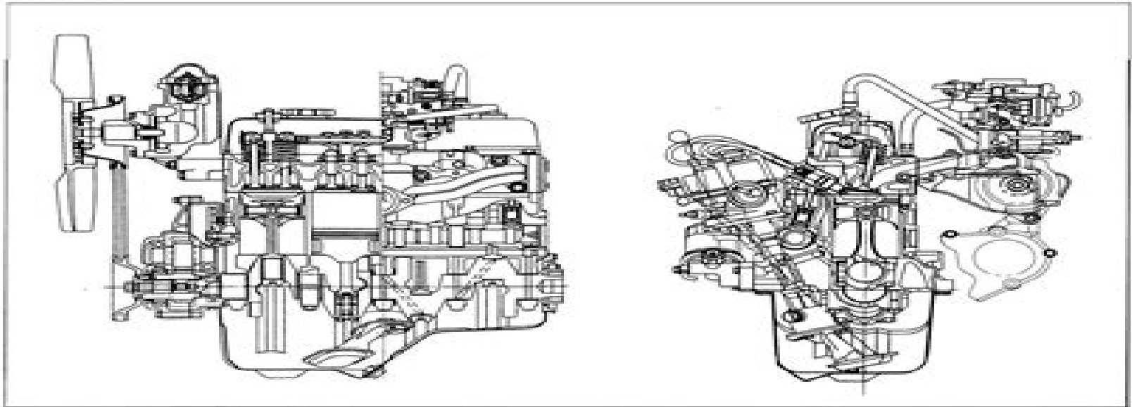
4Y Engine
