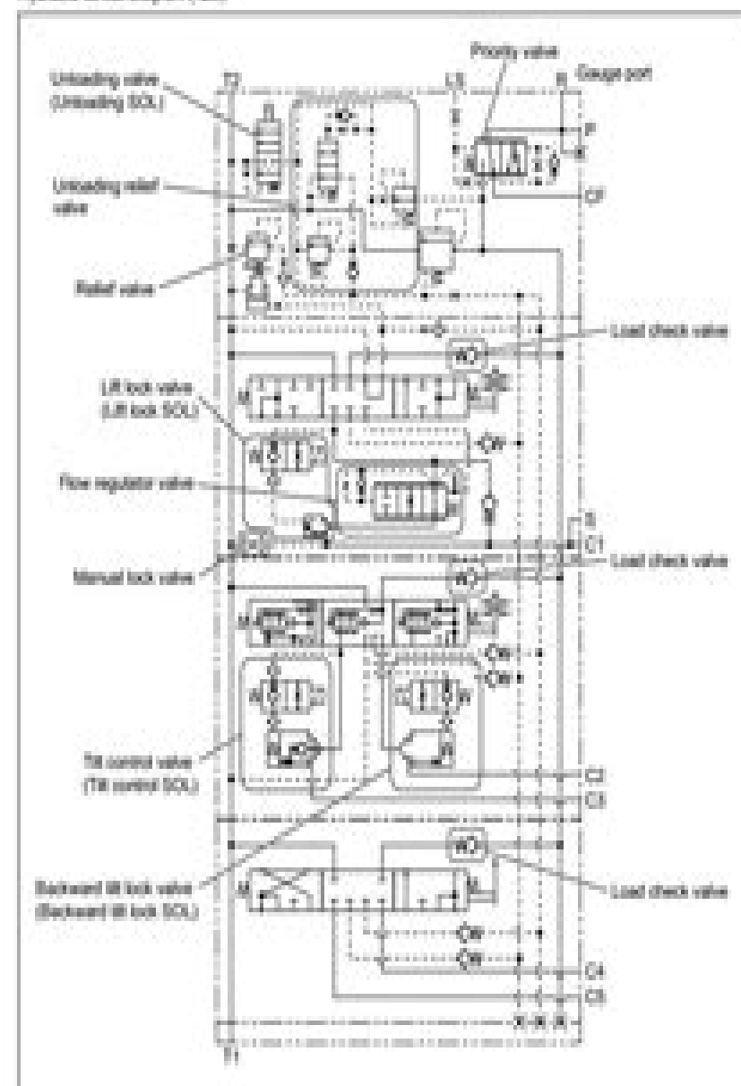
Hydraulic Circuit Diagram (125)
