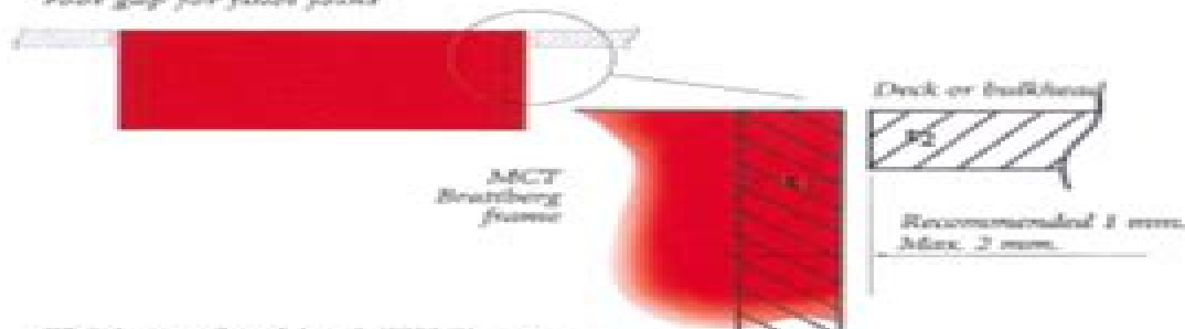
FIG 1: maximum allowable root gap for fillet joint
