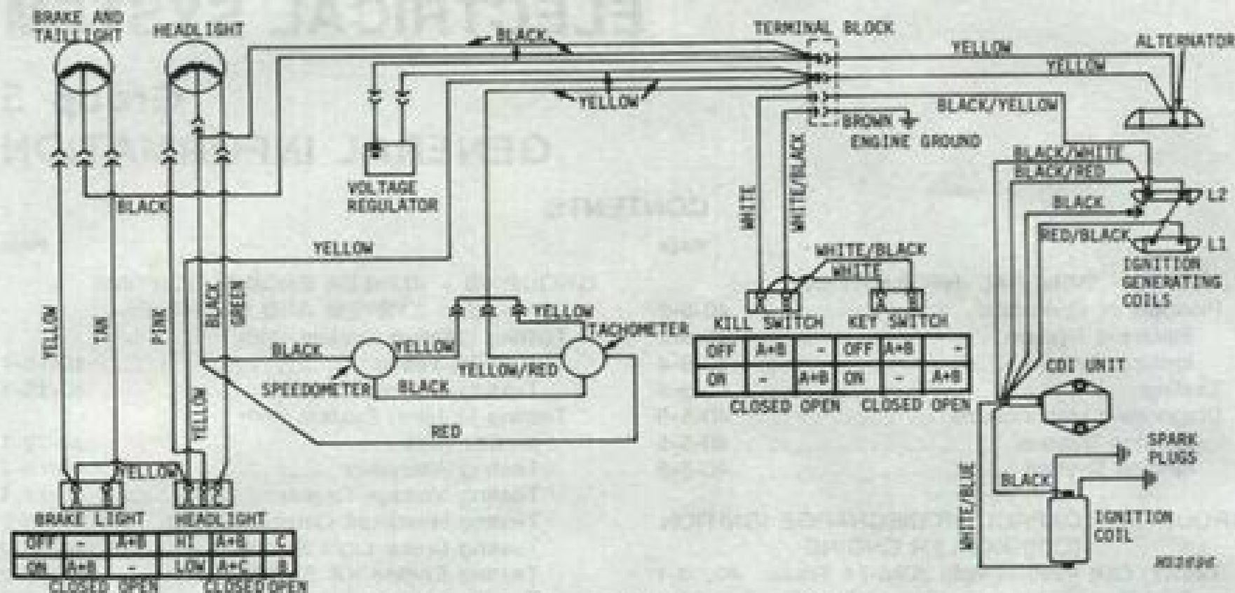
Fig. 1-Electrical System (Serial No. -120,000)
