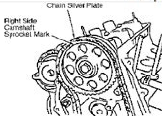
Fig. 11: Aligning Marks On Right 1st Timing Chain
