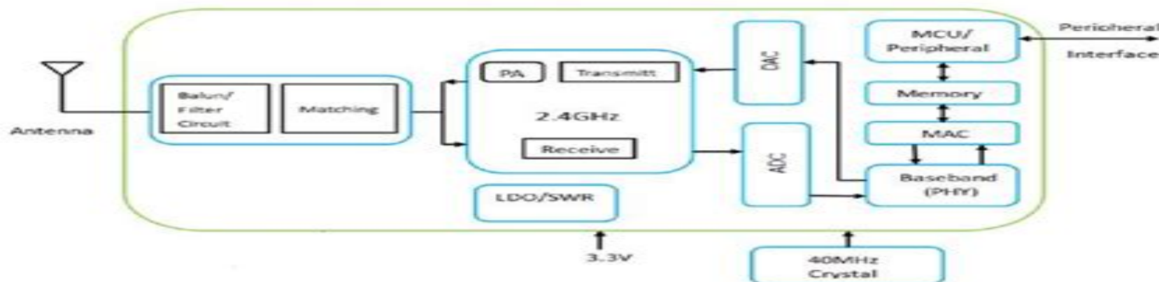
Figure 1-1 WBR3 architecture
