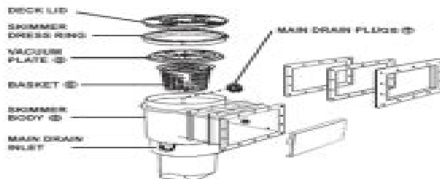
* Figure 3: S75 and Supaskimmer Skimmer Boxes
