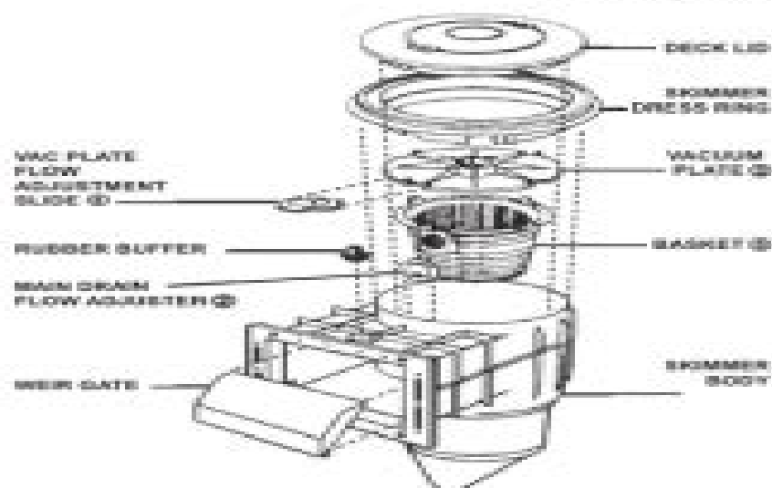
* Figure 1: SP5000 Skimmer Box
