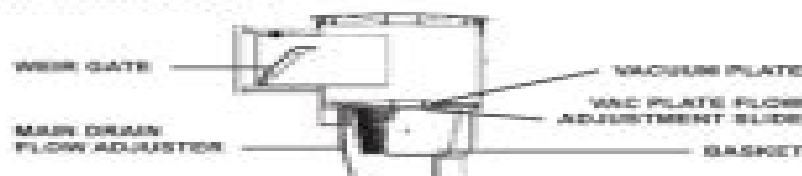
* Figure 2: XP5000 Skimmer Box (side view)
