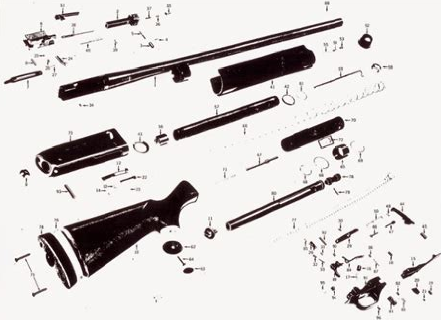
Diagram of a handgun showing the main components and their assembly sequence.
