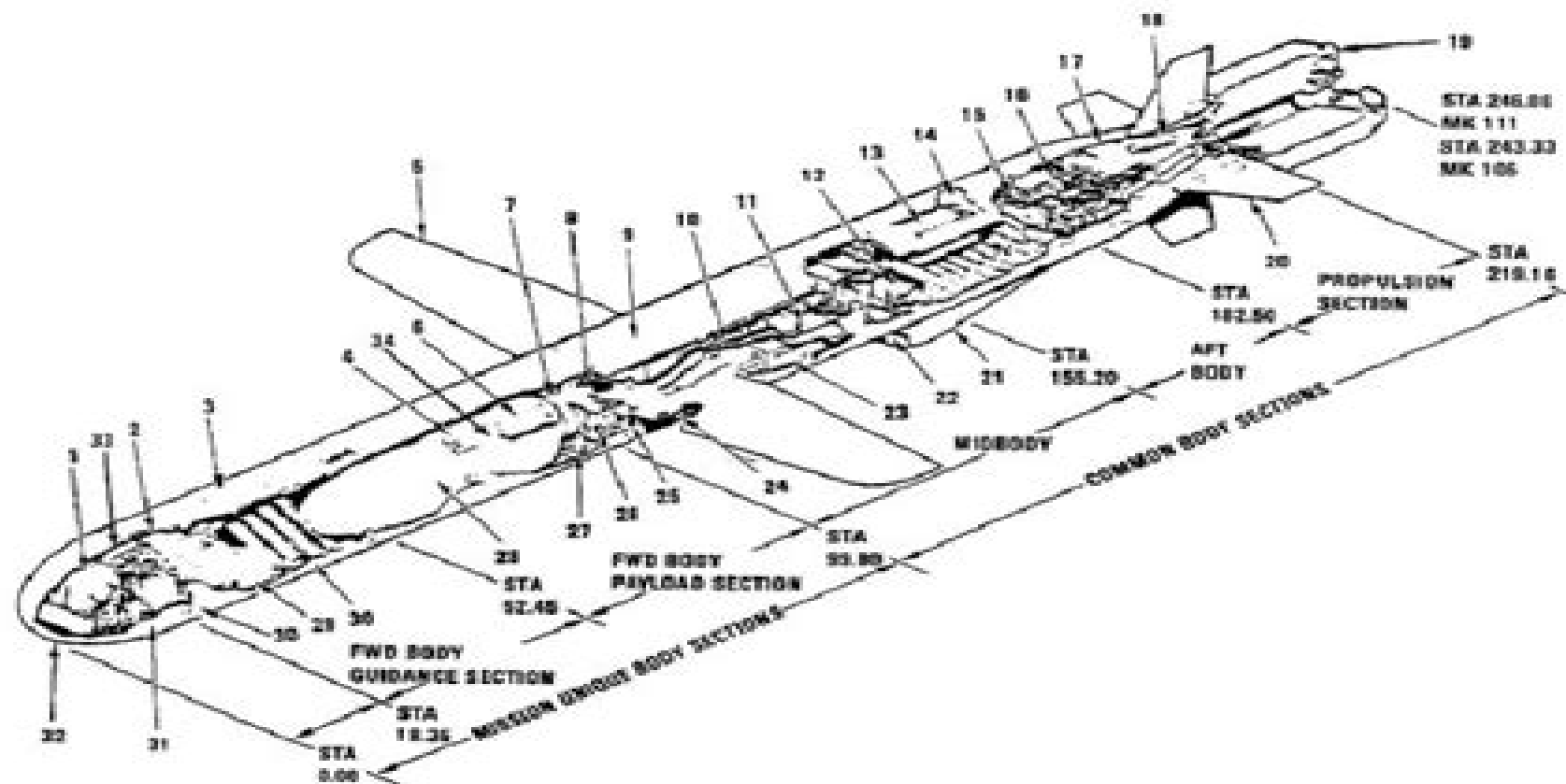
Figure 1-3. Land-Attack 109C
