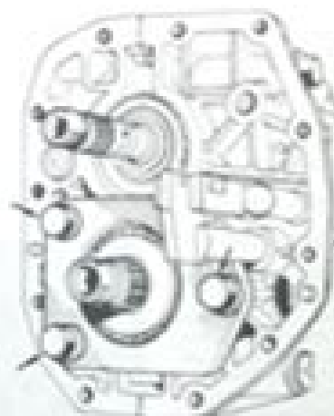
Fig. 6.21 Refit the bearing steel plate onto the rear face of the 368 gearbox (See 6)
