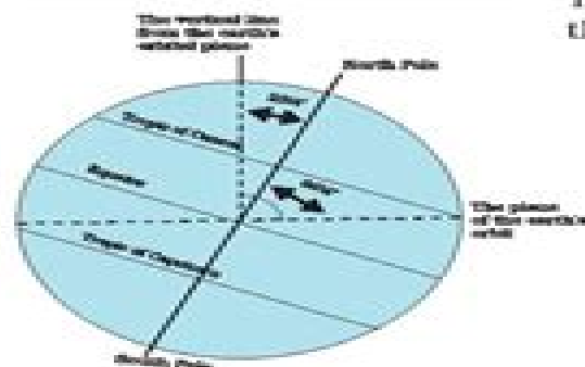
Figure 3.1 : Inclination of the Earth's axis and the orbital plane
