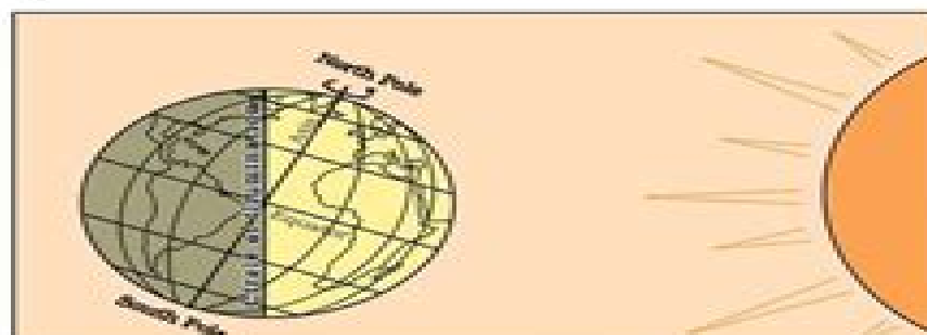
Figure 3.2 : Day and Night on the Earth due to rotation
