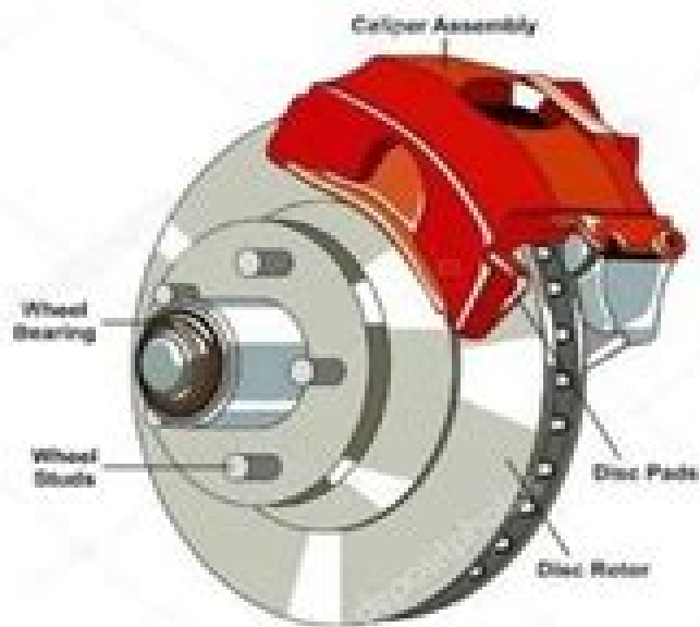
Disc Brake
