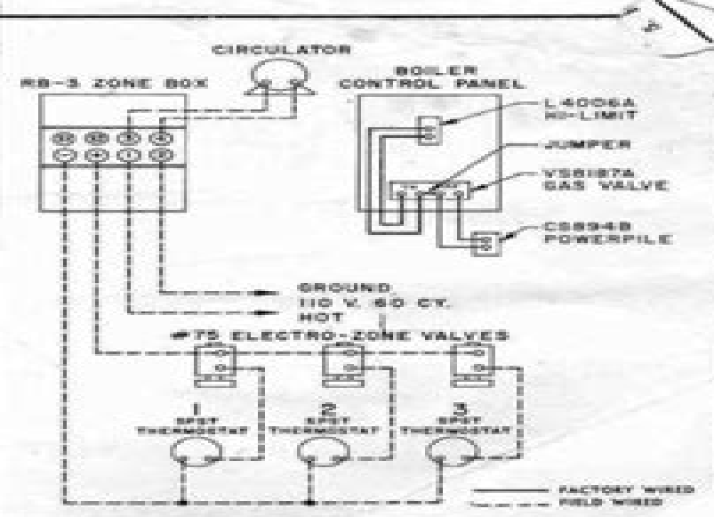
(Figure 5) THREE ZONES USING ELECTRO-ZONE VALV L4006A HIGH LIMIT AQUASTAT AND "RB-3"
