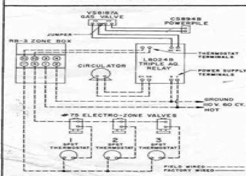
(Figure 4) THREE ZONE USING TRIPLE AQUASTAT RELAY AND "RB-3" ZONE BOX HY-P 234-1
