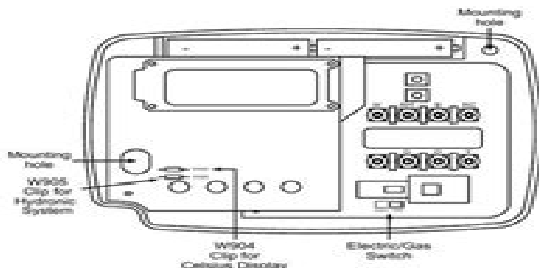
Figure 1. Thermostat base
