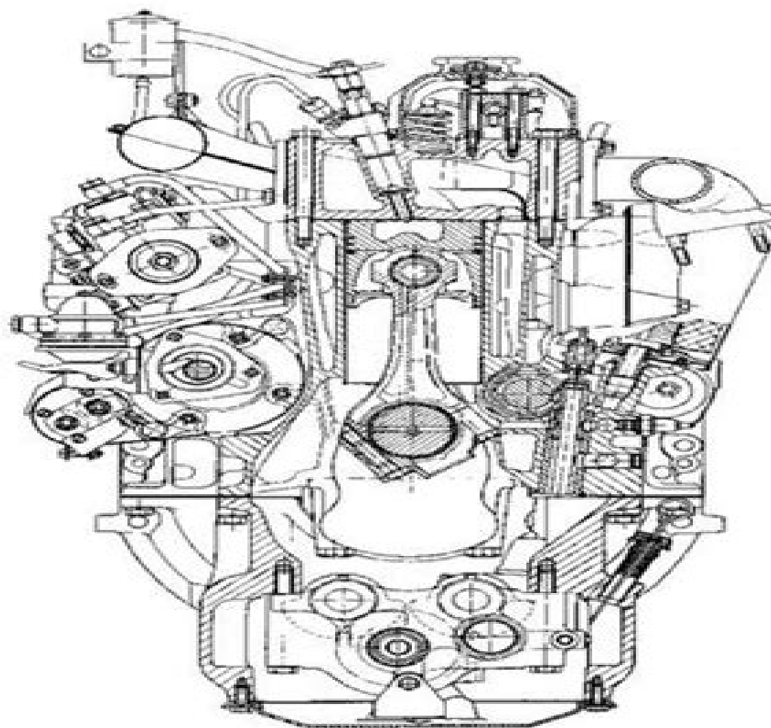
FIG. 2-11 Engine cut-section, end view.
