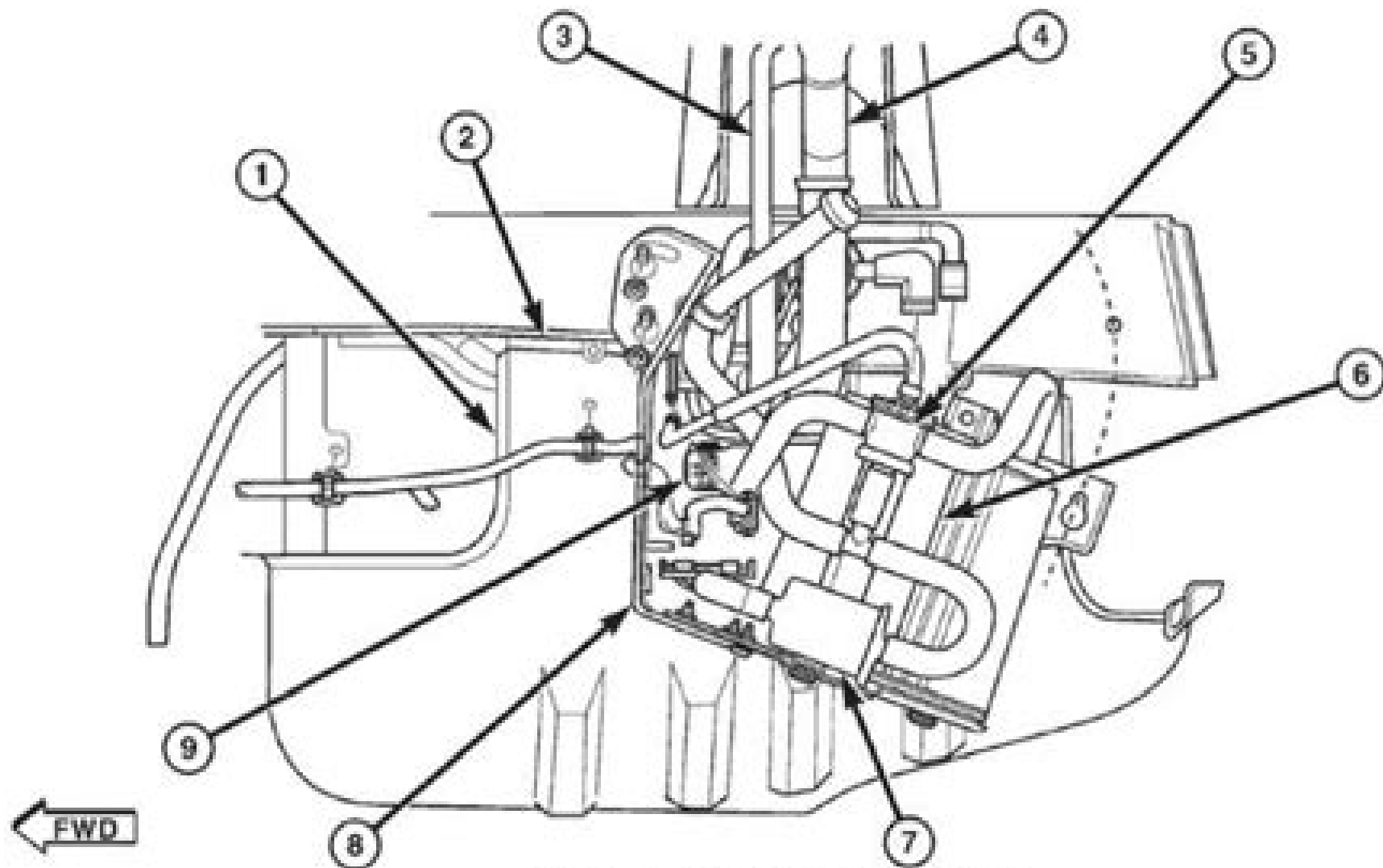
Fig. 1 ORVR / LDP COMPONENTS
