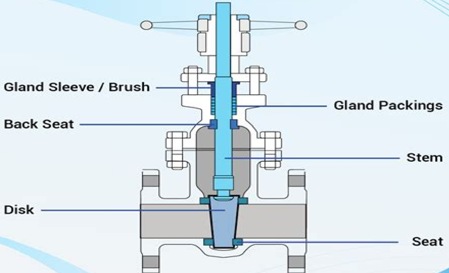
Valve Components
