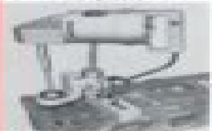
Photo 4—The H. O. Lee valve guide reaming tool is designed to remove any metal excess which does not valve guide as part of the cylinder head.
