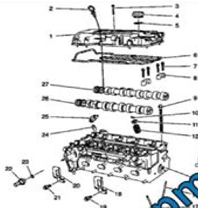
Fig. 6: Identifying Cylinder Head Assembly
