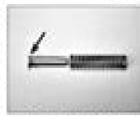
10.11c Ensure that the fuel side (arrowed) of the oil pump side gasket is facing forward (see 10.11a).
