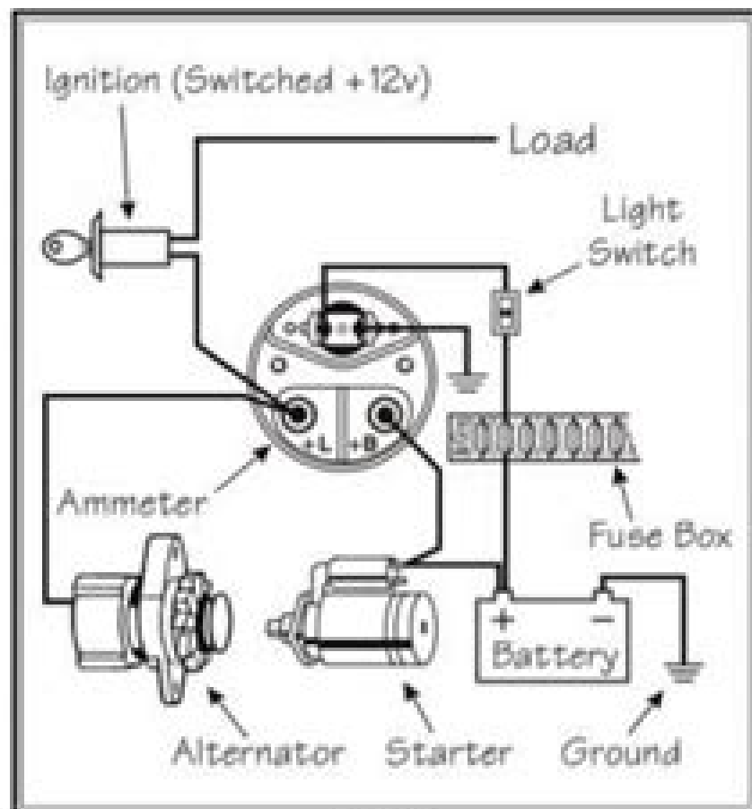
Diagram D Proper wiring of the VDO Ammeter
