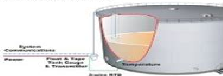
Example Tank Gauging System
