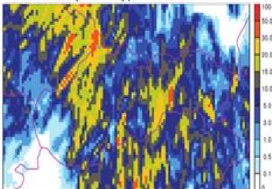
A-LAEF (EPS MAX) | 07/06/2020 12-15 UTC
