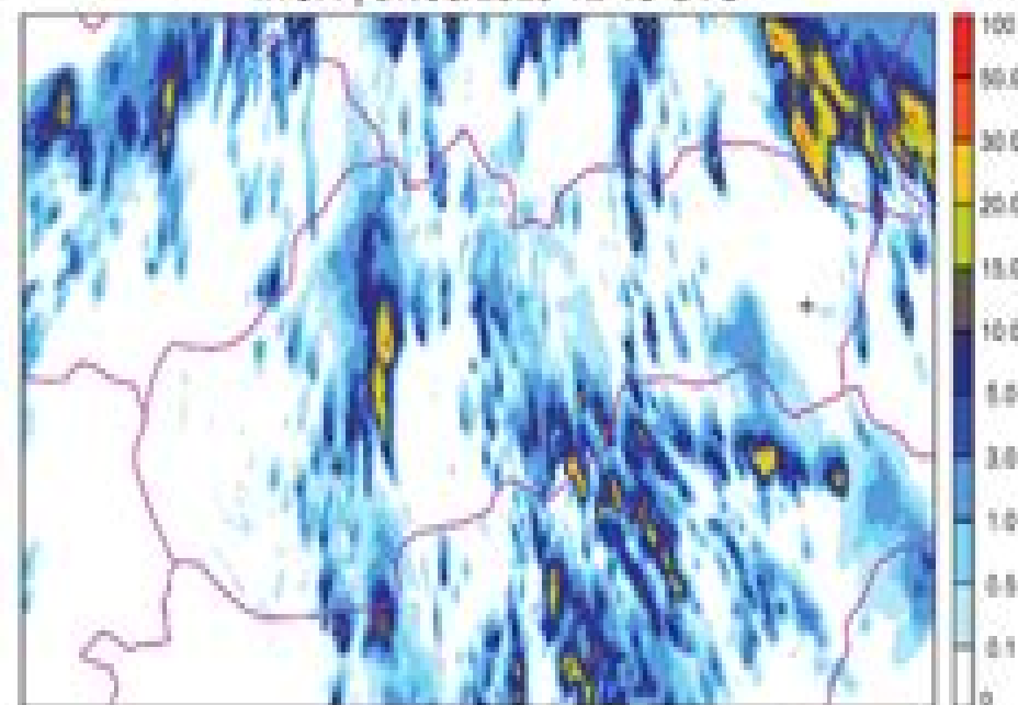
A-LAEF (EPS MEAN) | 07/06/2020 12-15 UTC
