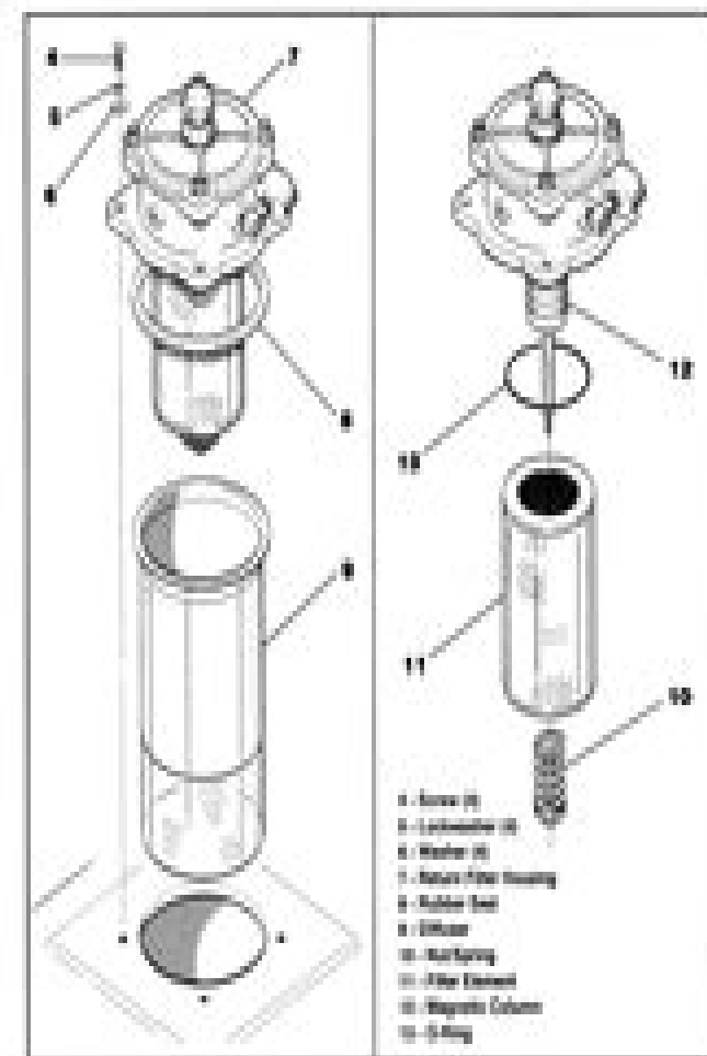
Figure 3-20 Filter Housing Assembly
