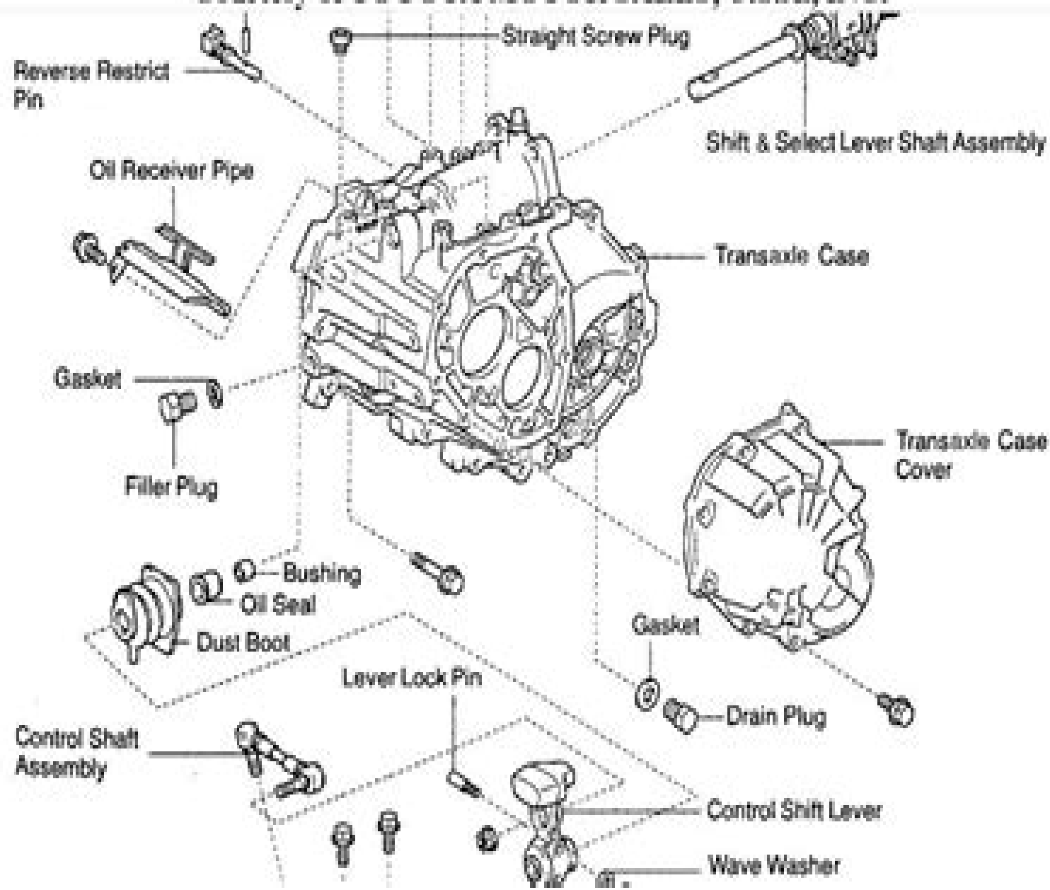
Fig. 1: Removing Transaxle Case External Components (Celica)
