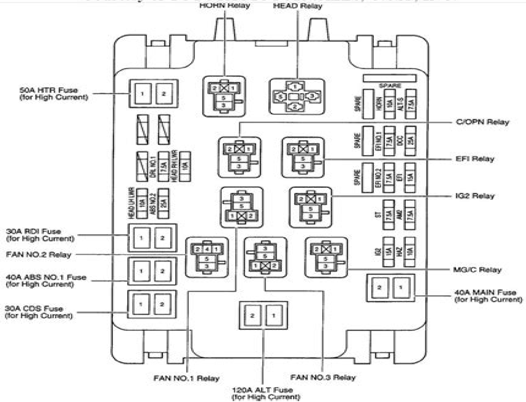
Fig. 9: Identifying Engine Room J/B Components Courtesy of TOYOTA MOTOR SALES, U.S.A., INC.
