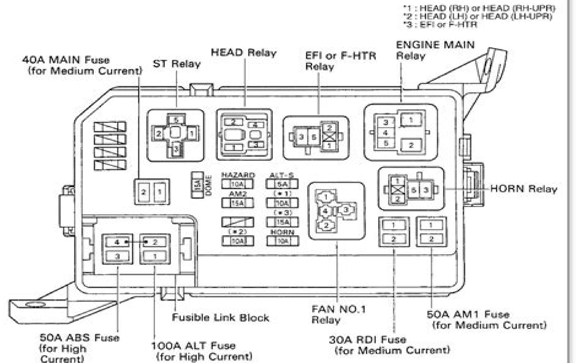
Fig. 15: Identifying Engine Room J/B Components
