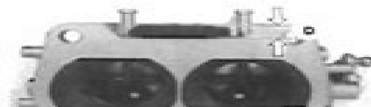
Fig. S218-2—Float height (D) should be 9.5-11.5 mm (0.37-0.45 in.). Bend tang on float arm to adjust.
