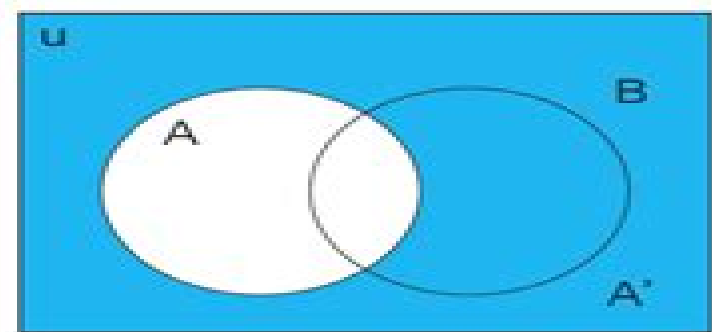
A' is the complement of A
