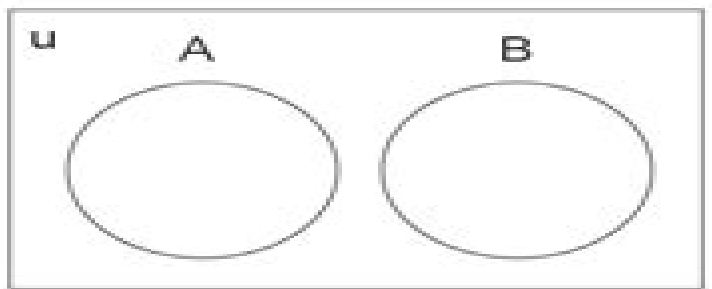
A and B are disjoint sets
