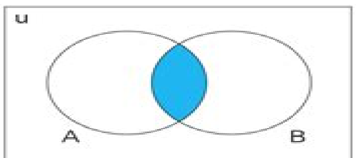
A \cap B A and B are overlapping sets
