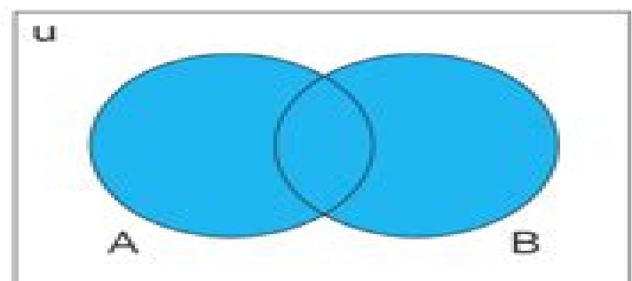
A \cup B A and B are overlapping sets
