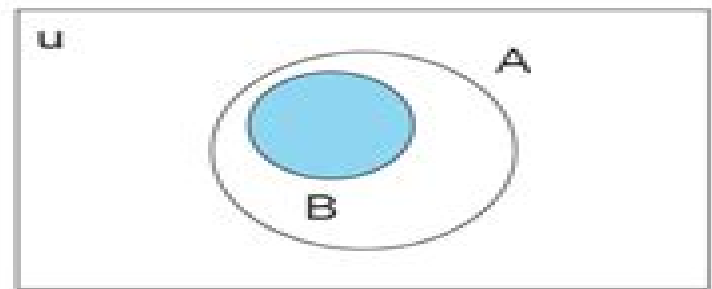
B \subset A B is proper subset of A
