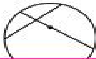
Intersecting Chords
