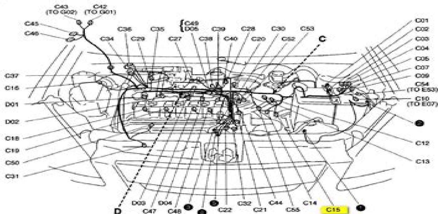
C: Engine harness
