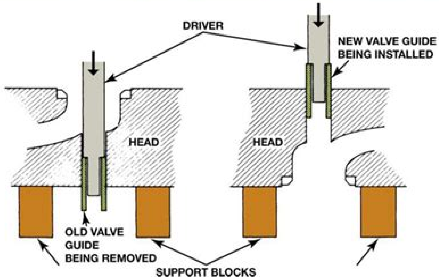
FIGURE 26–33 Valve guide replacement procedure.
