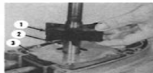
Fig. S218-20—View identifying water pump impeller (1), drive key (2) and plate (3).
