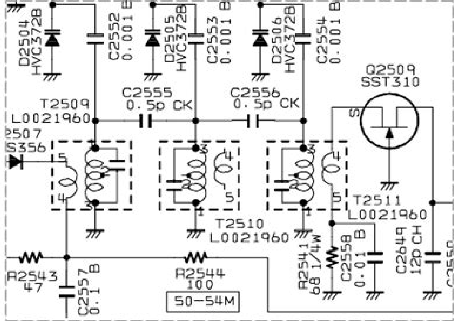
Preview: YAESU FT-DX9000 schematic diagram
