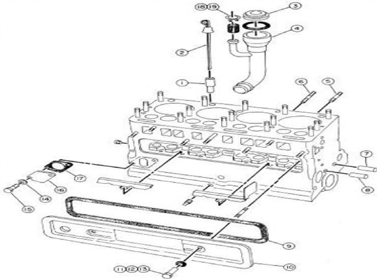
CYLINDER BLOCK GROUP T-7667
