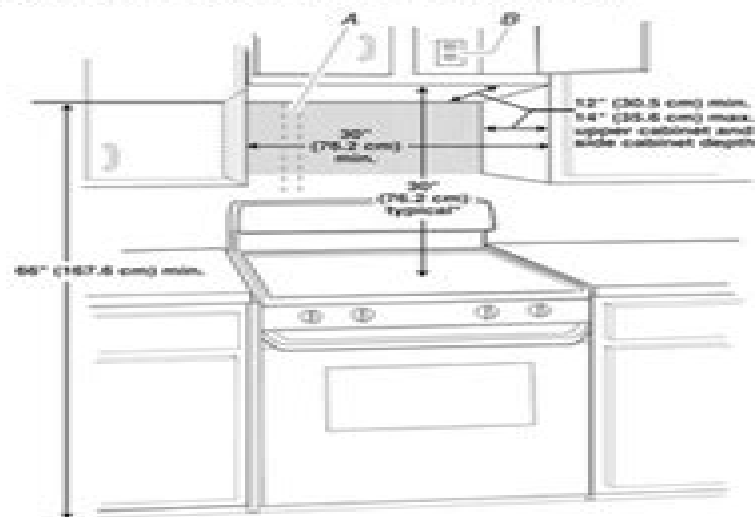
A. 2" x 4" (5.1 x 10.2 cm) wall stud B. Grounded 3 prong outlet
