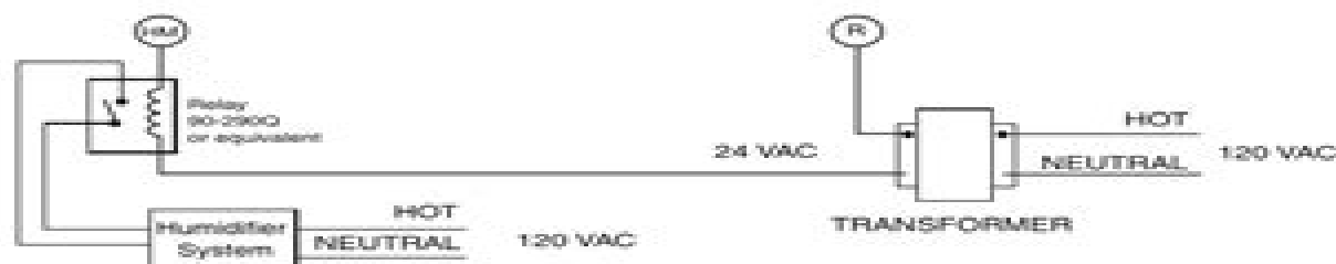
Figure 7 – Typical Wiring for 24V Humidifier System
