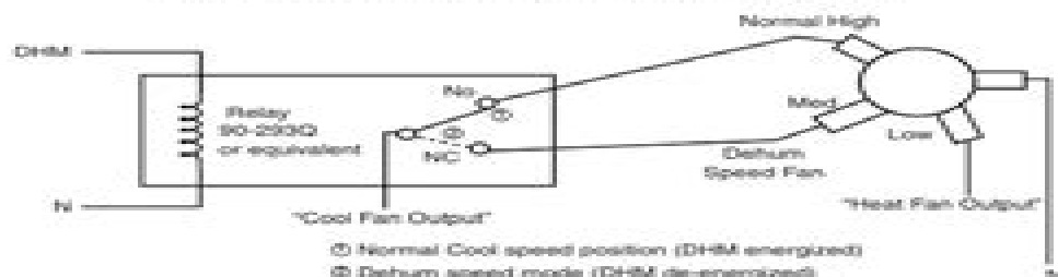
Figure 6 – Typical Wiring for 120V Humidifier System
