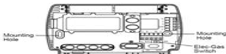
Figure 1 – Thermostat base
