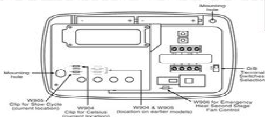
Figure 1. Thermostat base
